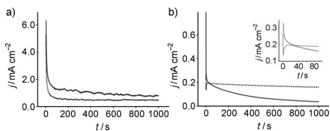
Figure 3. Chronoamperometric plots of MeOH oxidation at a) 0.50 V and b) 0.70 V on cubic \text{Pt}_3\text{Co} (—) and Pt NCBs (·····) in 0.1 M \text{HClO}_4 + 1 M MeOH. The inset in (b) is an enlargement of a shorter time section. Initial potential: 0.05 V.
